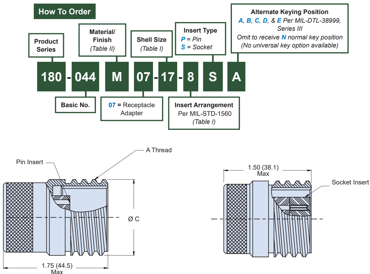
07 Receptacle Adapter U.S. PATENT NO. 5,960,137
