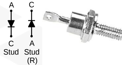
DO-4 Package
