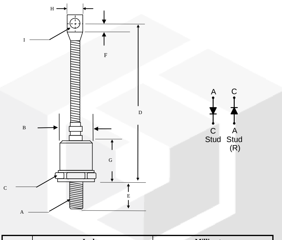
DO-8 (DO-205AA)
