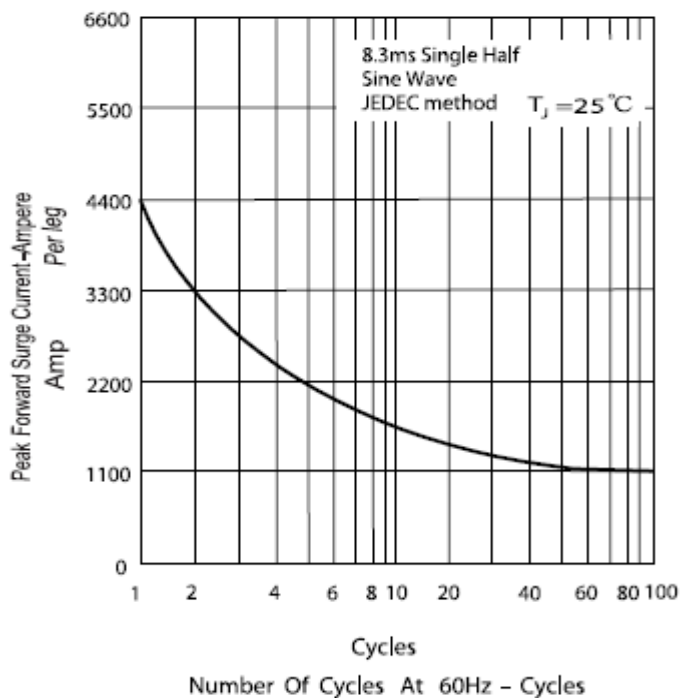
Figure .3- Peak Forward Surge Current
