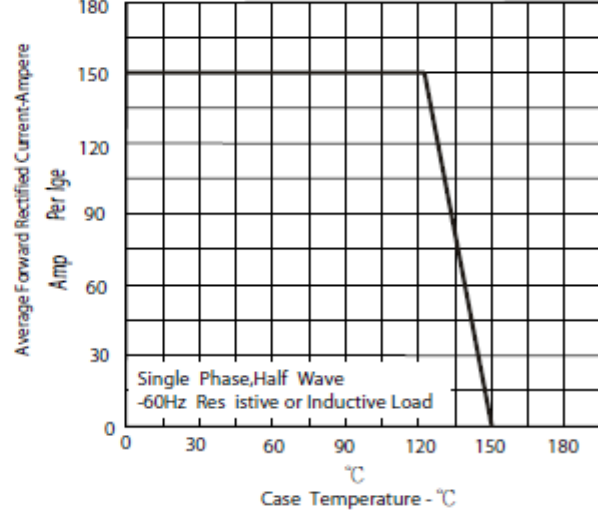
Figure.2-Forward Derating Curve
