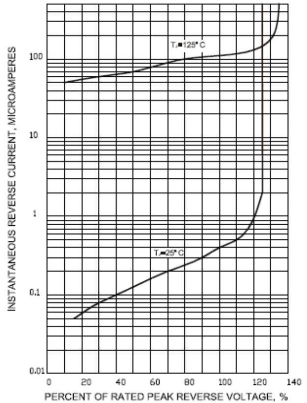
FIG.6-TYPICAL REVERSE CHARACTERISTICS
