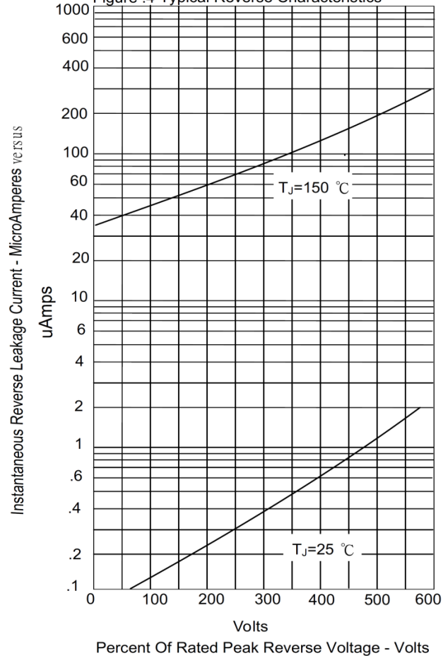
Figure .4-Typical Reverse Characteristics
