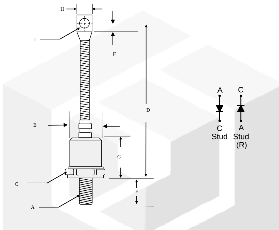
DO-8 (DO-205AA)
