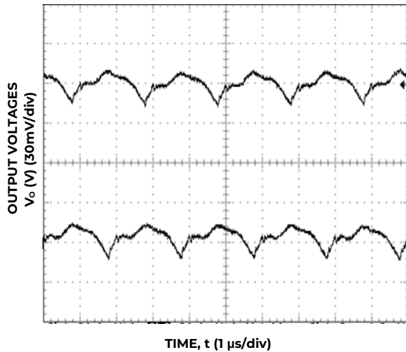
Figure 9. Typical output ripple and noise (C o = 2×0.1μF+2×47μF ceramic, V IN = 12V, I o = I o1,max , I o2,max ).
