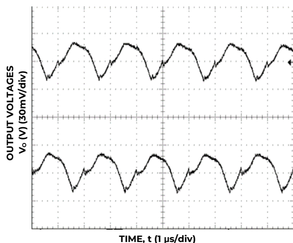
Figure 21. Typical output ripple and noise (C o = 2×0.1μF+2×47μF ceramic, V IN = 12V, I o = I o1,max , I o2,max ).
