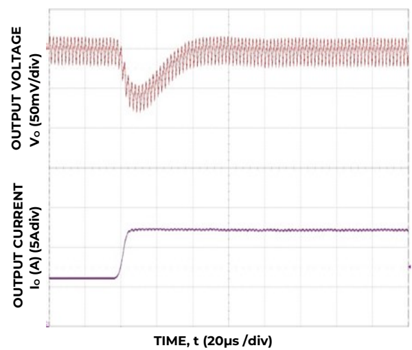
Figure 28 Transient Response to Dynamic Load Change on one output from 50% to 100% at 12V in , C_{out} = 3 \times 47\mu F + 1 \times 330\mu F , C_{Tune} = 1200pF & R_{Tune} = 300\Omega
