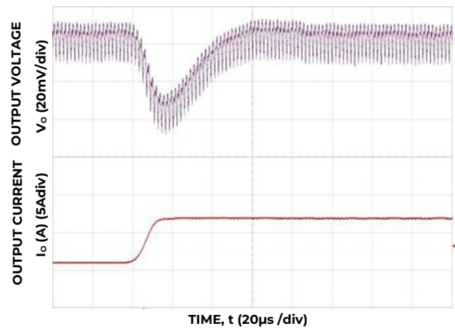
Figure 16. Transient Response to Dynamic Load Change from 50% to 100% on one output at 12V in , C_{out} = 3 \times 47\mu\text{F} + 3 \times 330\mu\text{F} , C_{Tune} = 1800\text{pF} & R_{Tune} = 300\Omega
