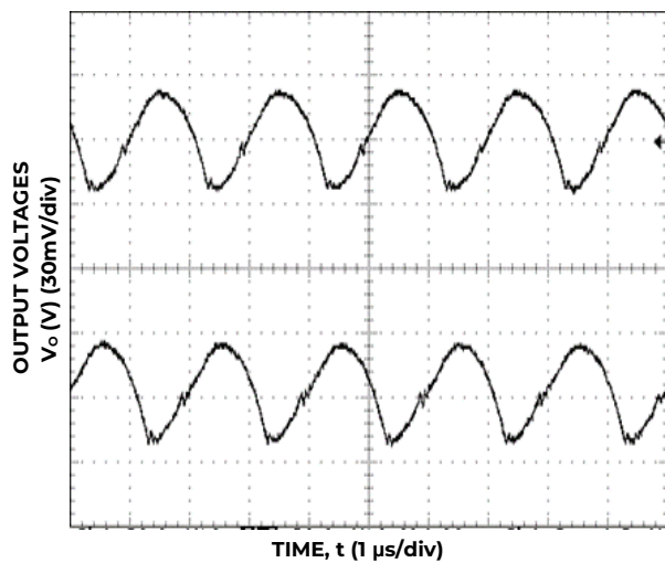
Figure 27. Typical output ripple and noise ( C_o = 2 \times 0.1\mu F + 2 \times 47\mu F ceramic, V_{IN} = 12V , I_o = I_{o1,max}, I_{o2,max} ).
