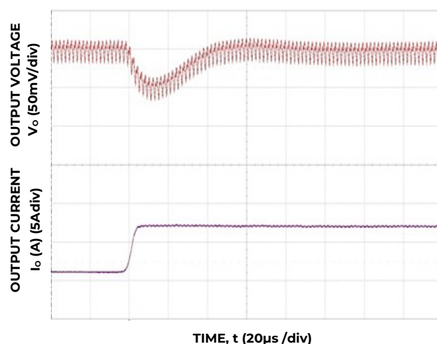
Figure 22. Transient Response to Dynamic Load Change from 50% to 100% on one output at 12V in , C out = 3×47μF+3×330μF, C Tune = 1500pF & R Tune = 300Ω
