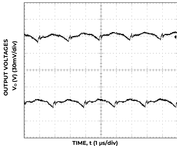
Figure 3. Typical output ripple and noise ( C_o = 2 \times 0.1\mu F + 2 \times 47\mu F ceramic, V_{IN} = 12V , I_o = I_{o1,max}, I_{o2,max} ).
