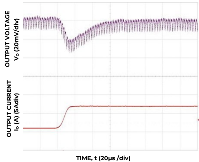
Figure 10. Transient Response to Dynamic Load Change from 50% to 100% on one output at 12V in , C out =3×47μF+3×330μF, C Tune =2700pF & R Tune =300Ω
