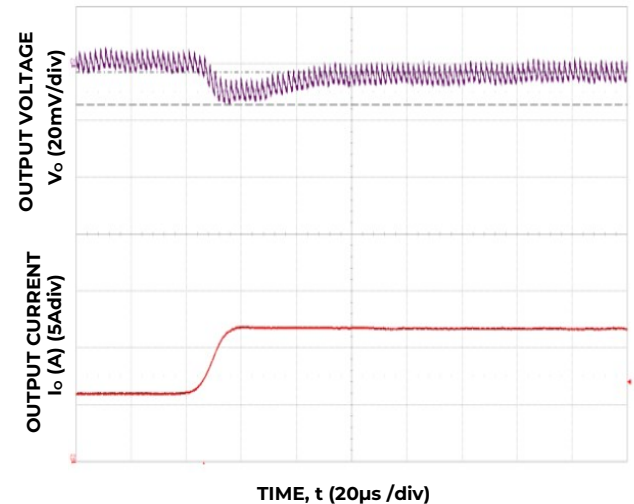
Figure 4. Transient Response to Dynamic Load Change from 50% to 100% on one output at 12V in , C_{out} = 2 \times 47\mu F + 7 \times 330\mu F , C_{Tune} = 12nF , R_{Tune} = 300\Omega
