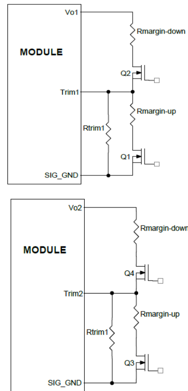
Figure 43. Circuit Configuration for margining Output voltage.
