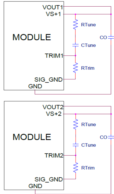
Figure 47. Circuit diagram showing connection of R_{TUNE} and C_{TUNE} to tune the control loop of the module.
