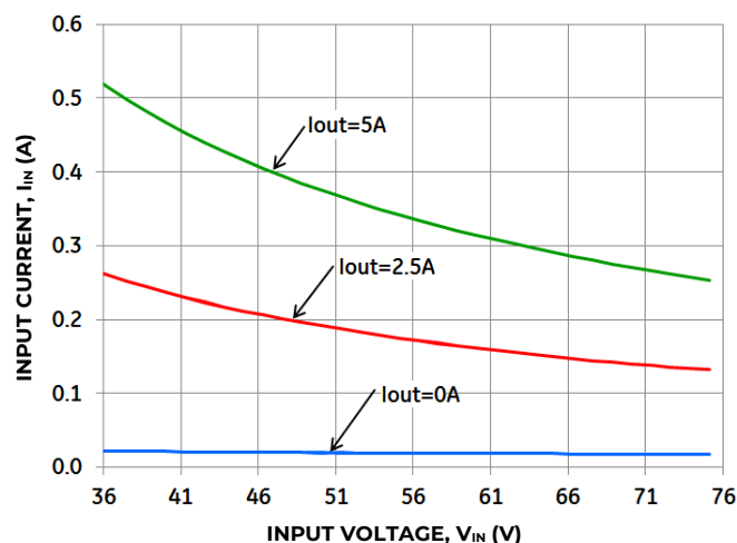
Figure 2. Converter Input Current versus Input Voltage.
