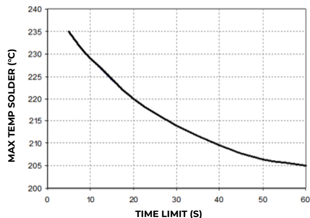
Figure 20 Time Limit, T_{lim} , Curve Above 205 °C Reflow.
