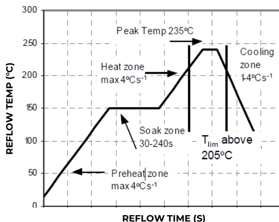
Figure 20. Recommended Reflow Profile for Sn/Pb solder.
