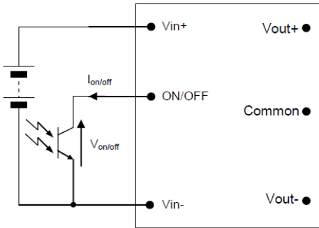
Figure 11. Circuit configuration for using Remote On/Off Implementation.
