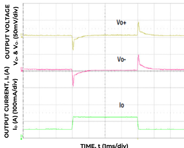
Figure 4. Transient Response to 0.1A/μs Dynamic Load Change from 50% to 75% to 50% of full load, V_{in}=24V .
