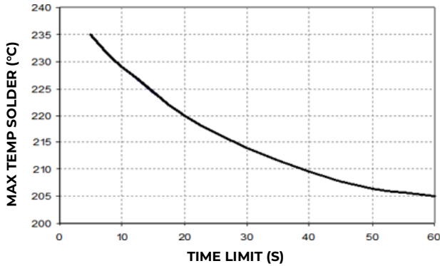
Figure 22. Time Limit, T_{lim} , Curve Above 205 °C Reflow .
