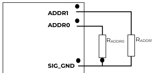
Figure 24. Circuit showing connection of resistors used to set the PMBus address of the module.
