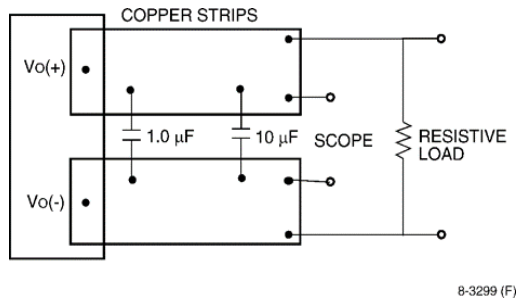
Figure 11. Input Reflected Ripple Current Test Setup.
