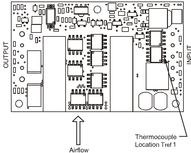
Figure 38. Temperature Measurement Location.
