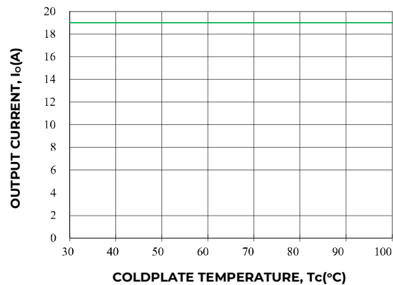
Figure 21. Derated Output Current versus Cold Wall Temperature with local ambient temperature around module at 75^{\circ}C ; V_{IN} = 24V or 48V .
