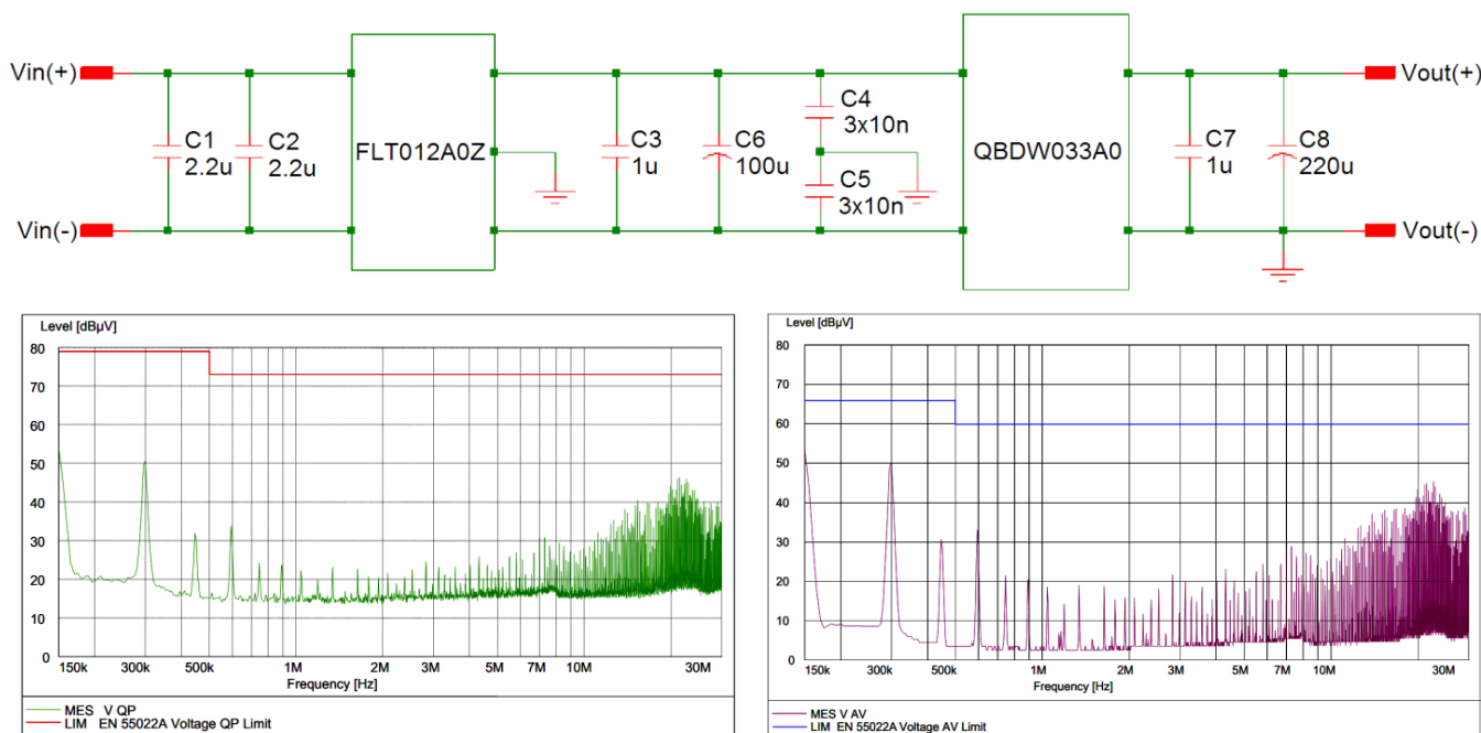
Figure 25. EMC Consideration
