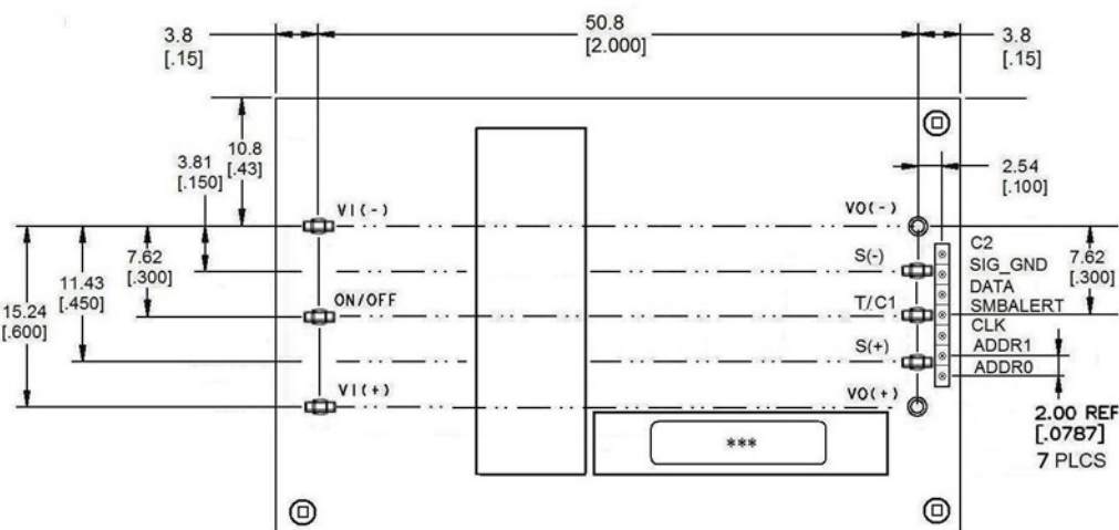
BOTTOM VIEW
