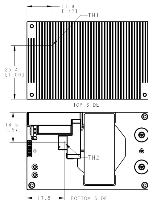
Figure 16. Location of the thermal reference temperature TH1 and TH2 for integrated heatsink module.
