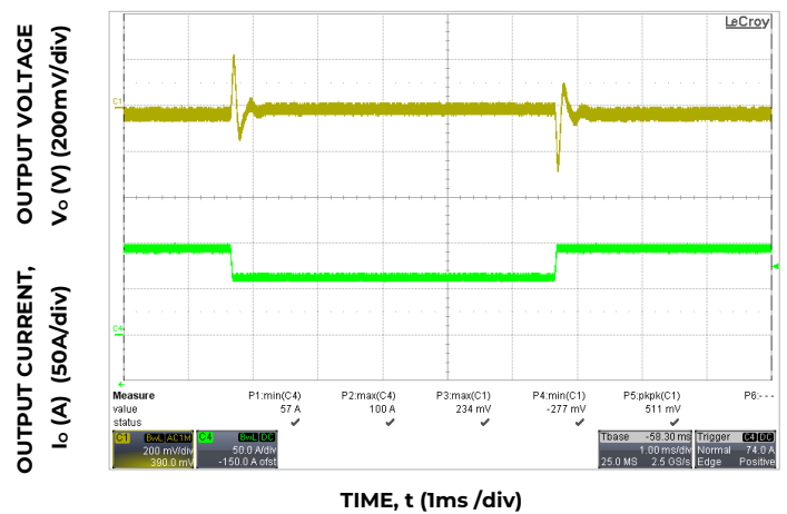
Figure 4. Dynamic Load Response, di_o/dt=1A/\mu s ; V_{in}=V_{in,nom} ; T_A=25^\circ C ; Load Change from I_o = 50\% to 75\% of I_{o,max} ; Co = 5200uF Ceramic;
