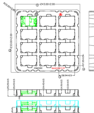
Base Plate Module Tray
