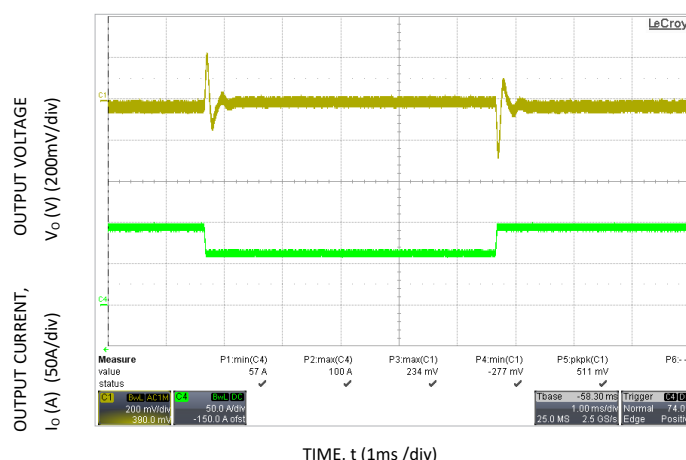
Figure 4. Dynamic Load Response, di_o/dt=1A/us ; V_{in}=V_{in,nom} ; T_A=25^\circ C ; Load Change from I_o = 50\% to 75\% of I_{o,max} ; C_o = 5200\mu F Ceramic;
