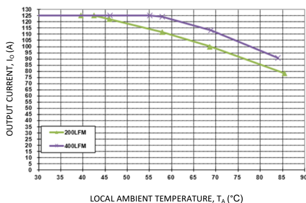
Figure 18. Output Current Derating for the Base plate QBDS125A10R4-H+0.6" Heat Sink; Airflow Direction for Vout to Vin(Worst) orientation; Vin = 54V.
