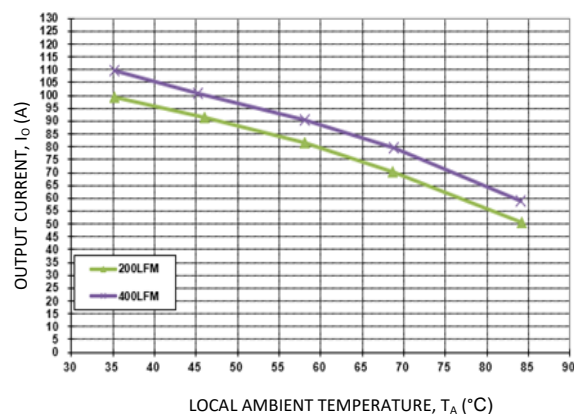
Figure 15. Output Current Derating for the Base Plate QBDS125A10R4-H; Airflow Direction for Vout to Vin(Worst) orientation; Vin = 50V.
