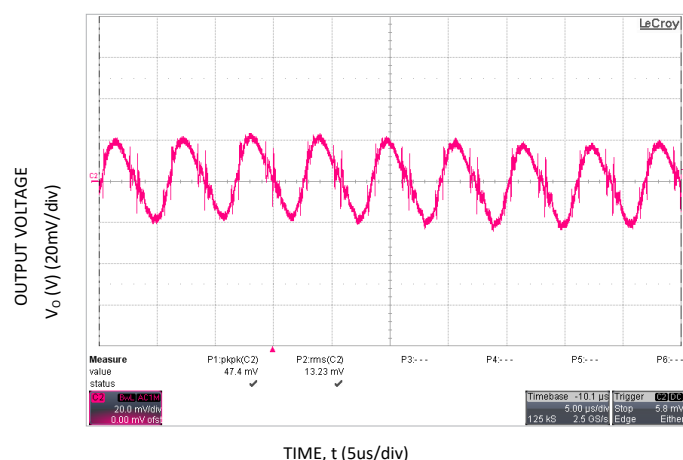
Figure 3. Typical output ripple and noise ( C_o = 650\mu F Ceramic + 650\mu F PosCap Oscon, V_{in} = 54V , I_o = I_{o,max} ).
