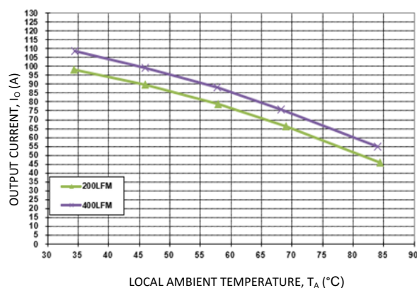
Figure 16. Output Current Derating for the Base Plate QBDS125A10R4-H; Airflow Direction for Vout to Vin(Worst) orientation; Vin = 54V.
