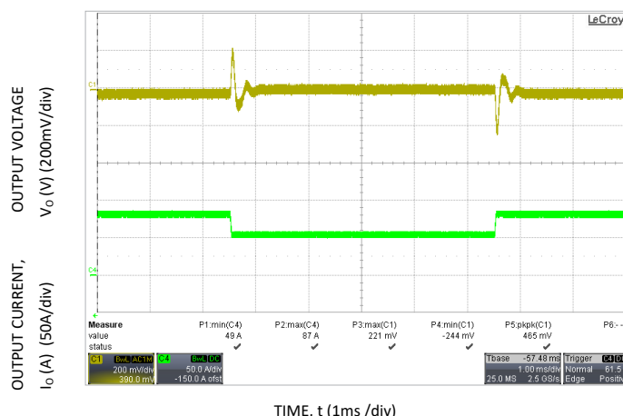
Figure 4. Dynamic Load Response, di_o/dt=1\text{A}/\mu\text{s} ; V_{in}=V_{in,nom} ; T_A=25^\circ\text{C} ; Load Change from I_o = 50\% to 75\% of I_{o,max} ; C_o = 5200\mu\text{F} Ceramic;
