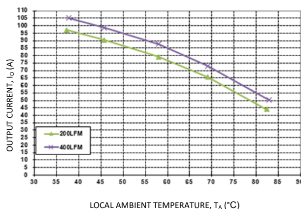
Figure 16. Output Current Derating for the Base Plate QBDS108A0B-H; Airflow Direction for Vout to Vin(Worst) orientation; Vin = 54V.
