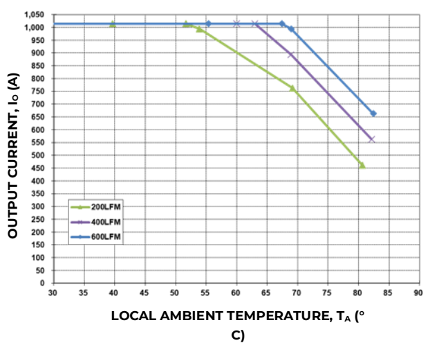
Figure 18. Output Current Derating for the Base plate QBDS095A10R6-H+0.6" Heat Sink; Airflow Direction for Vout to Vin (Worst) orientation; Vin = 54V.
