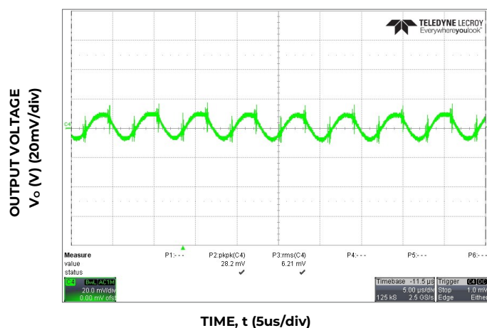
Figure 3. Typical output ripple and noise ( C_o = 500\mu\text{F} Ceramic + 500\mu\text{F} PosCap Oscon, V_{in} = 56\text{V} , I_o = I_{o,max} ).
