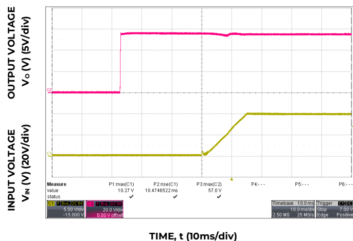
Figure 6. Typical Start-up Using Input Voltage ( V_{in} = 56\text{V} , I_o = I_{o,max} ).
