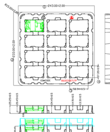
Base Plate Module Tray Figure 27. QBDS095A10R6 Packaging Tray
