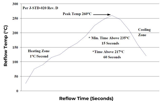
Figure 48. Recommended linear reflow profile using Sn/Ag/Cu solder.
