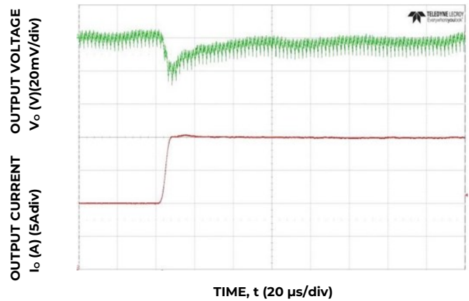
Figure 10. Transient Response to Dynamic Load Change from 50% to 100% at 12V in , C out = 7x47μF + 4x330 μF, C Tune =6800pF, R Tune =300
