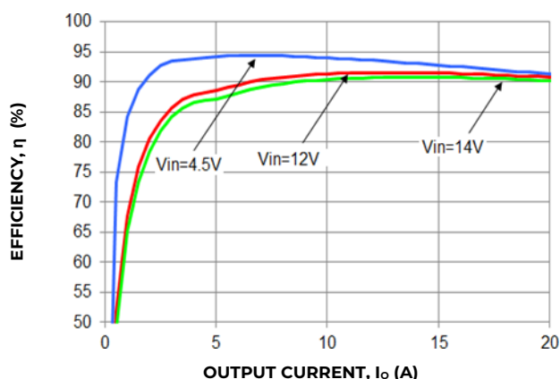
Figure 13. Converter Efficiency verses output current
