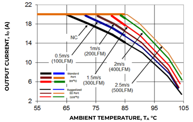
Figure 8. Derating Output Current verses Ambient Temperature and Airflow.
