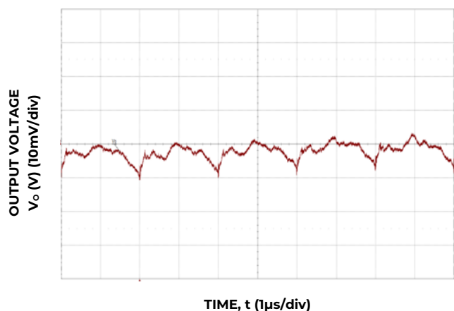
Figure 3. Typical output ripple (C o =7x22μF ceramic, V IN = 12V, I o = I o,max ).
