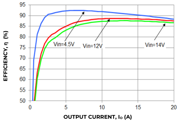
Figure 7. Converter Efficiency verses output current
