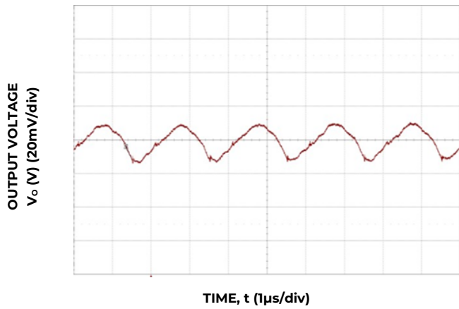
Figure 27. Typical output ripple and noise ( C_o=7x22\mu F ceramic, V_{IN} = 12V , I_o = I_{o,max} ).
