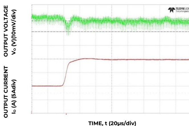
Figure 4. Transient Response to Dynamic Load Change from 50% to 100% at 12V in , C out = 7x47μF + 9x330μF, C Tune =15nF, R Tune =300
