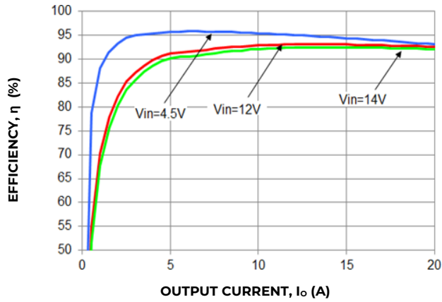
Figure 19. Converter Efficiency verses output current
