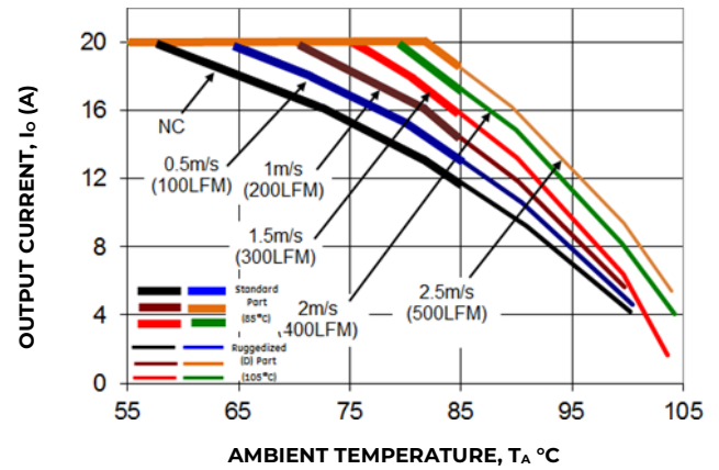
Figure 20. Derating Output Current verses Ambient Temperature and Airflow.
