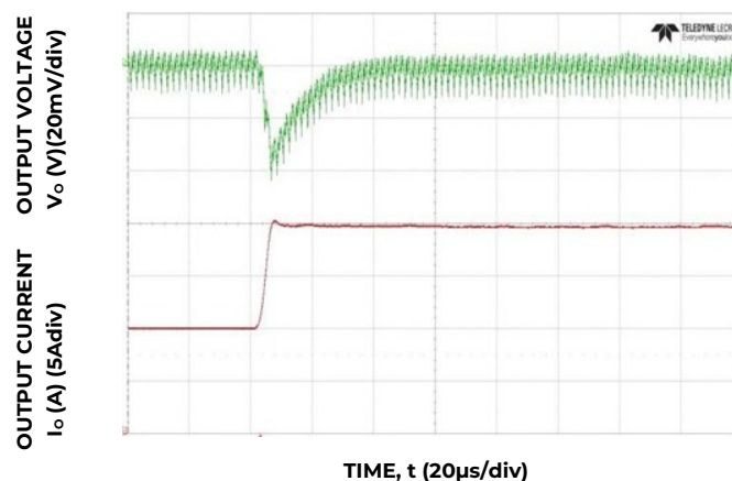
Figure 16. Transient Response to Dynamic Load Change from 50% to 100% at 12V in , C out = 7x47μF + 2x330μF, C Tune =3900pF
