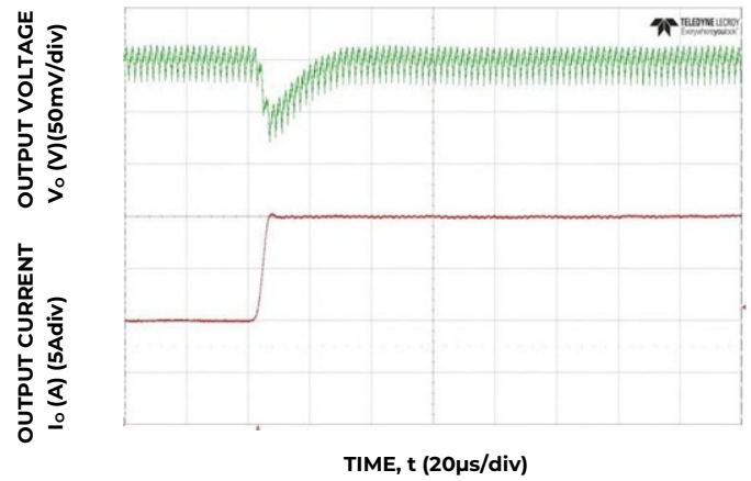
Figure 28. Transient Response to Dynamic Load Change from 50% to 100% at 12V in , C_{out} = 4x47\mu F + 1x330\mu F , C_{Tune}=1800 pF
