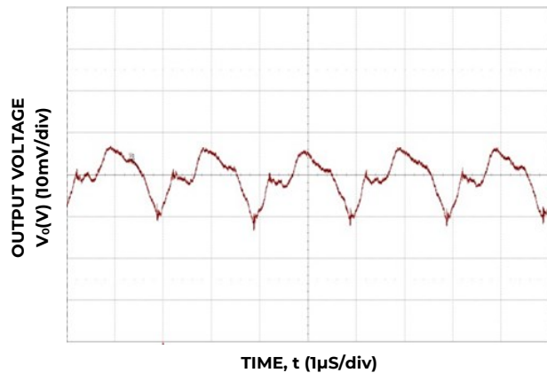
Figure 15. Typical output ripple ( C_o = 7 \times 22 \mu\text{F} ceramic, V_{IN} = 12\text{V} , I_o = I_{o,max} ).
