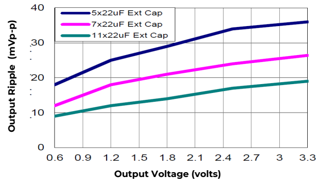
Figure 32. Output ripple voltage for various output voltages with external 5x22 \mu F, 7x22 \mu F or 11x22 \mu F ceramic capacitors at the output (20A load). Input voltage is 12V.
