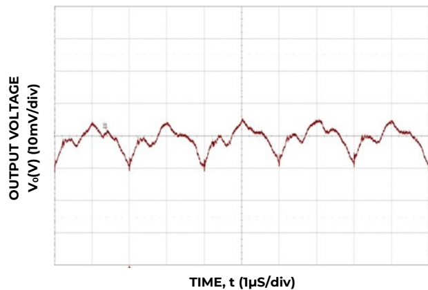
Figure 9. Typical output ripple ( C_o=7 \times 22\mu\text{F} ceramic, V_{IN} = 12\text{V} , I_o = I_{o,max} ).
