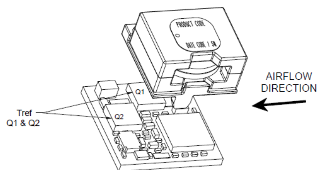
Figure 43. Preferred airflow direction and location of hot-spot of the module ( T_{ref} ).
