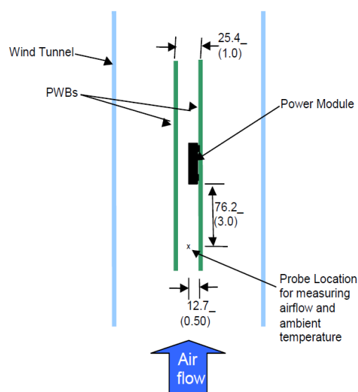
Figure 42. Thermal Test Setup.
