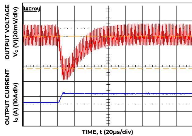
Figure 16. Transient Response to Dynamic Load Change from 50% to 100% at 12V in , C out =1x47μF+2x330μF, C Tune =5600pF, R Tune =270ohms
