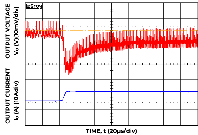
Figure 10. Transient Response to Dynamic Load Change from 50% to 100% at 12V in , C out =1x47μF+3x330μF, C Tune =10nF, R Tune =220ohms
