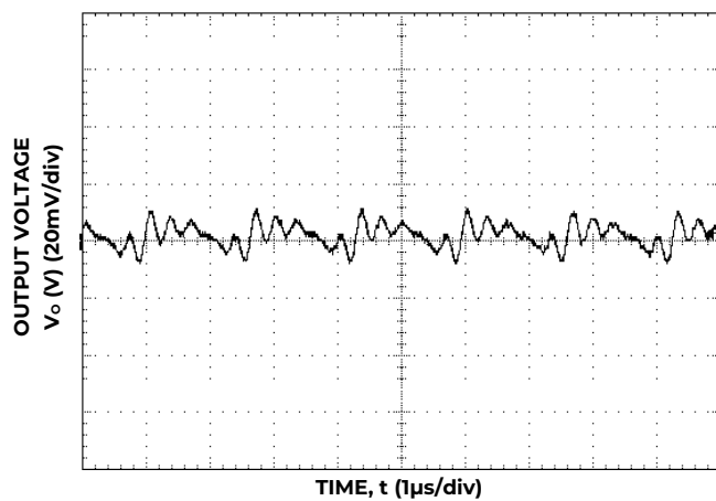
Figure 9. Typical output ripple and noise (C o =22μF ceramic, V IN = 12V, I o = I o,max ).
