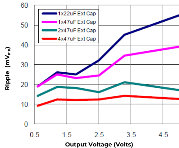
Figure 38. Output ripple voltage for various output voltages with external 1x22 \mu F, 1x47 \mu F, or 4x47 \mu F ceramic capacitors at the output (12A load). Input voltage is 12V.
