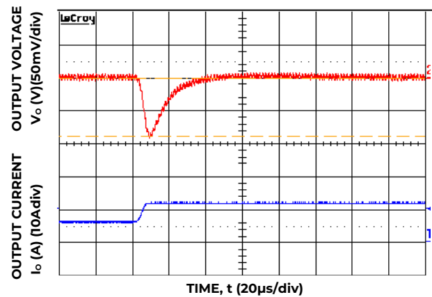
Figure 34. Transient Response to Dynamic Load Change from 50% to 100% at 12V in , C out =5x47μF, C Tune =1500pF, R Tune =330 ohms
