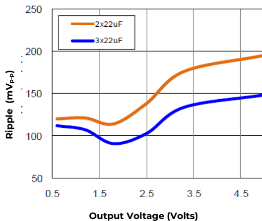
Figure 37. Input ripple voltage for various output voltages with 2x22 \mu F or 3x22 \mu F ceramic capacitors at the input (12A load). Input voltage is 12V.
