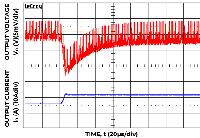
Figure 4. Transient Response to Dynamic Load Change from 50% to 100% at 12V in , C out =3x47uF+6x330uF, C Tune =47nF, R Tune =180ohm
