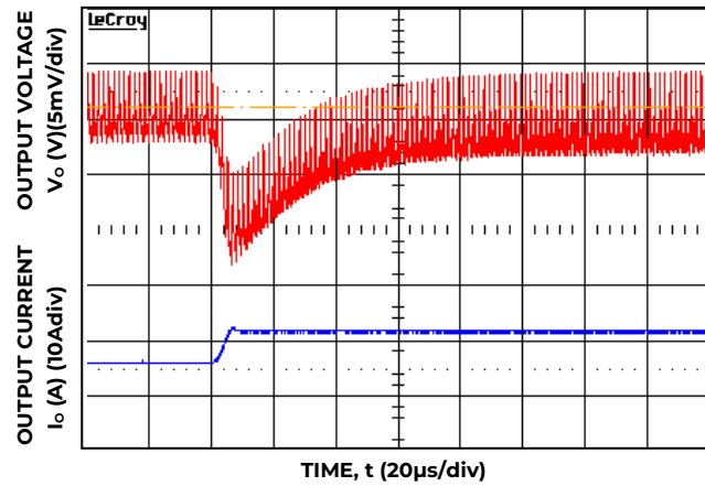
Figure 4. Transient Response to Dynamic Load Change from 50% to 100% at 12V in , C out =3x47μF+6x330μF, C Tune =47nF, R Tune =180ohm.
