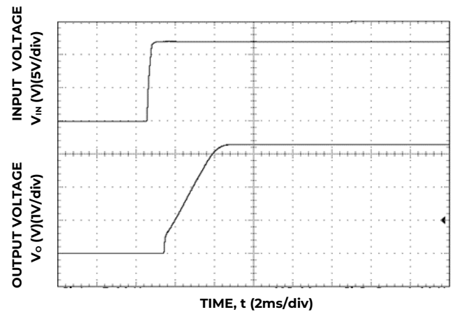
Figure 30. Typical Start-up Using Input Voltage ( V_{IN}=12\text{V} , I_o=I_{o,max} ).
