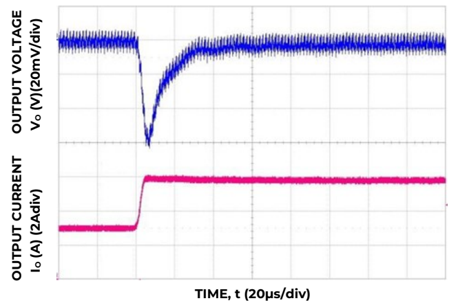
Figure 28. Transient Response to Dynamic Load Change from 50% to 100% at 12V in , C_{out}=3 \times 47\mu\text{F} , C_{Tune}=3300\text{pF} , R_{Tune}=178
