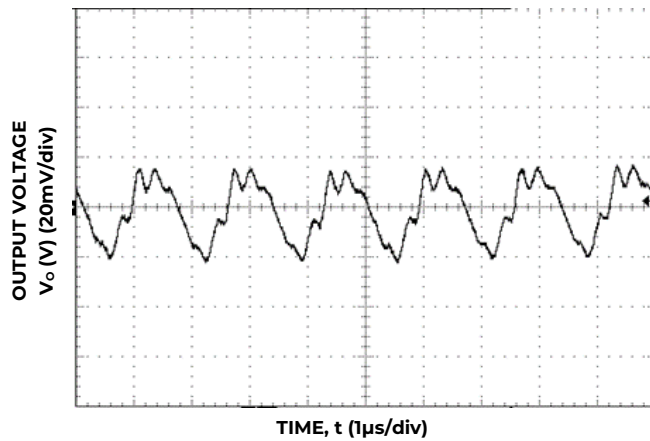
Figure 27. Typical output ripple and noise ( C_O=2 \times 47\mu\text{F} ceramic, V_{IN}=12\text{V} , I_o=I_{o,max} ).
