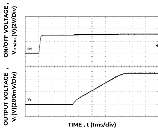
Figure 35. Typical Start-up Using On/Off Voltage ( I_o = I_{o,max} ).
