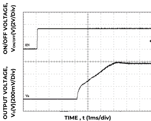
Figure 5. Typical Start-up Using On/Off Voltage ( I_o = I_{o,max} ).
