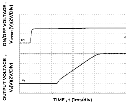
Figure 41. Typical Start-up Using On/Off Voltage ( I_o = I_{o,max} ).
