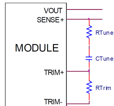
Figure 51. Circuit diagram showing connection of R_{\text{TUNE}} and C_{\text{TUNE}} to tune the control loop of the module.
