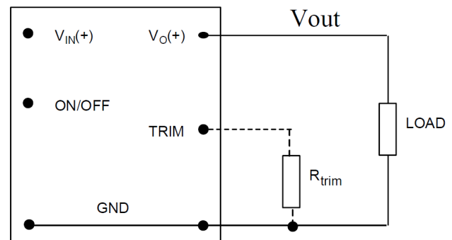
Figure 49. Circuit configuration for programming output voltage using an external resistor.
