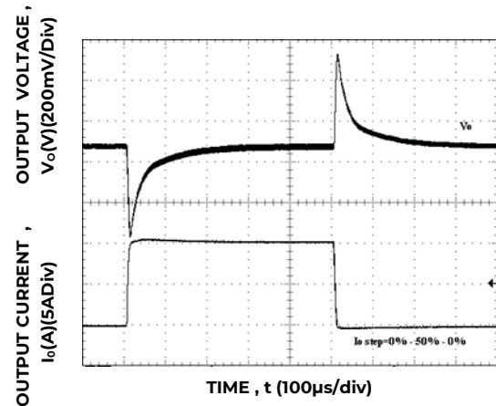
Figure 40. Transient Response to Dynamic Load Change from 0% to 50% to 0% with V_{IN}=12V .
