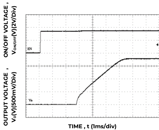
Figure 17. Typical Start-up Using On/Off Voltage ( I_o = I_{o,max} ).
