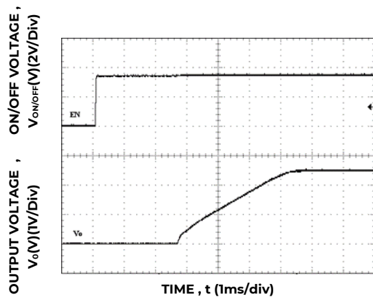
Figure 23. Typical Start-up Using On/Off Voltage (I o = I o,max ).
