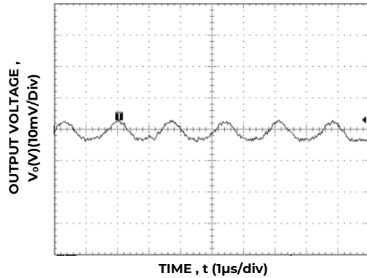
Figure 3. Typical output ripple and noise ( V_{IN} = 9V , I_o = I_{o,max} ).
