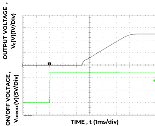
Figure 23. Typical Start-up Using On/Off Voltage ( I_o = I_{o,max} ).
