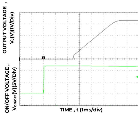
Figure 29. Typical Start-up Using On/Off Voltage ( I_o = I_{o,max} ).
