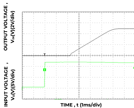
Figure 42. Typical Start-up Using Input Voltage (V IN = 12V, I o = I o,max ).
