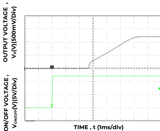
Figure 11. Typical Start-up Using On/Off Voltage (I o = I o,max ).
