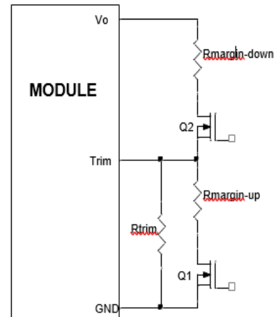
Figure 51. Circuit Configuration for margining Output voltage.
