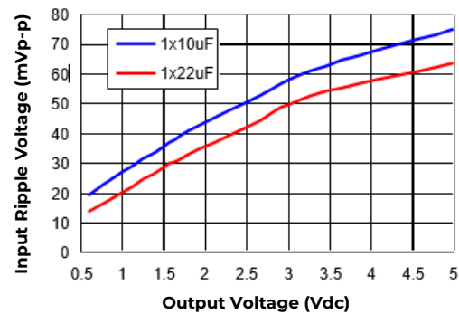
Figure 46. Input ripple voltage for various output voltages with 1 \times 10 \mu F or 1 \times 22 \mu F ceramic capacitors at the input (3A load). Input voltage is 12V
