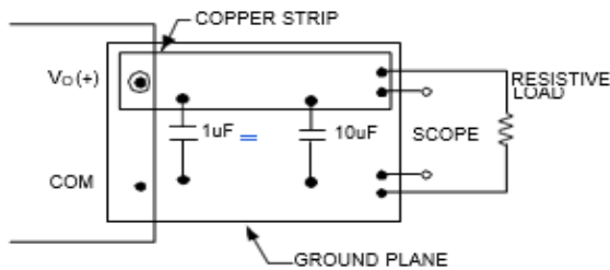
Figure 44. Output Ripple and Noise Test Setup
