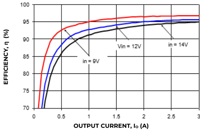
Figure 37. Converter Efficiency versus Output Current.
