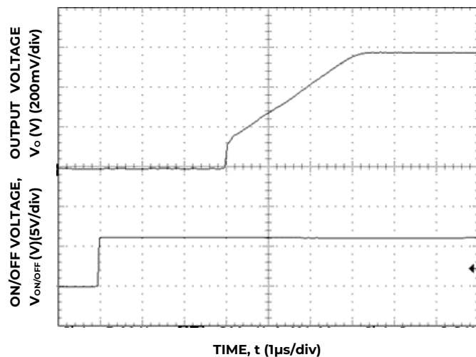
Figure 5. Typical Start-up Using On/Off Voltage ( I_o = I_{o,max} ).
