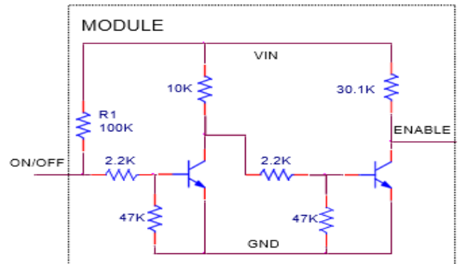
Figure 48. Remote On/Off Implementation. Resistor R1 is absent in the -49Z option module.
