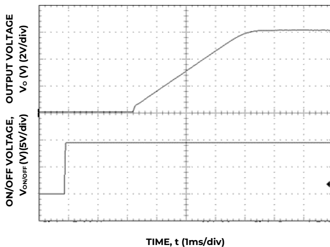
Figure 41. Typical Start-up Using On/Off Voltage ( I_o = I_{o,max} ).
