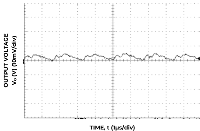
Figure 3. Typical output ripple and noise ( V_{IN} = 9V , I_o = I_{o,max} ).
