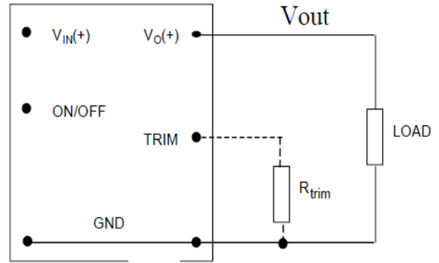
Figure 50. Circuit configuration for programming output voltage using an external resistor.
