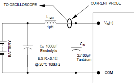
Figure 43. Input Reflected Ripple Current Test Setup.
