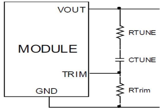
Figure 52. Circuit diagram showing connection of R_{TUNE} and C_{TUNE} to tune the control loop of the module.
