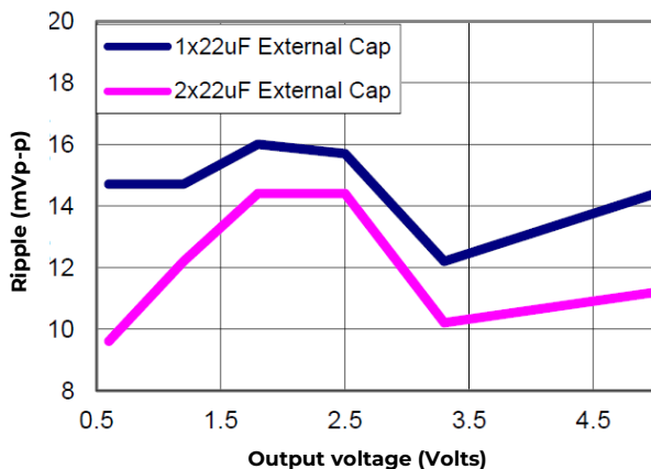
Figure 5. Output ripple voltage for various output voltages with external 1x22 \mu F, 2x22 \mu F ceramic capacitors at the output (2A load). Input voltage is 12V.
