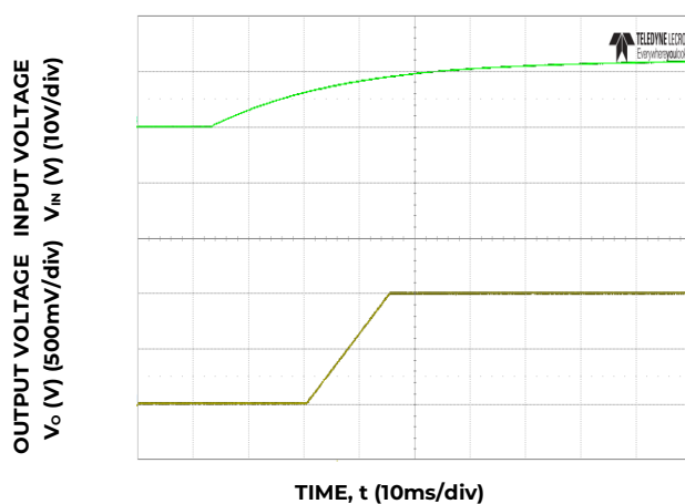
Figure 12. Typical Start-up Using Input Voltage ( V_{IN}=12\text{V} , I_o=I_{o,max} ).
