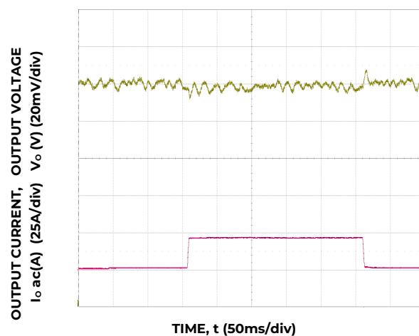
Figure10. Trans. Resp. to 10A/ \mu\text{s} Load Change from 25% to 75% at 12VIN, C_o=4\times0.047\mu\text{F}+4\times0.1\mu\text{F}+15\times22\mu\text{F}+73\times47\mu\text{F}+6\times470\mu\text{F} polymer
