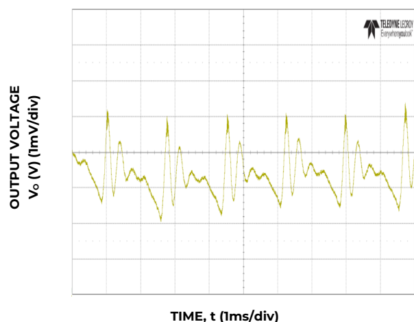
Figure 9. Typical output ripple( C_o=4\times0.047\mu\text{F}+4\times0.1\mu\text{F}+15\times22\mu\text{F}+73\times47\mu\text{F}+6\times470\mu\text{F} polymer, V_{IN}=12\text{V} , I_o=I_{o,max} ).
