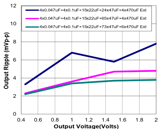
Figure 26. Peak to peak output ripple voltage for various output voltages with external capacitors at the output (40A load). Input voltage is 12V.
