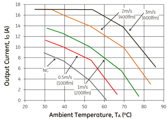
Figure 20. Derating Output Current vs. Ambient temperature and Airflow, No Heatsink, V_{IN}=48\text{V} , airflow from V_i(-) to V_i(+) .
