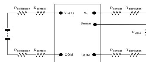
Figure 33. Remote sense circuit configuration.
