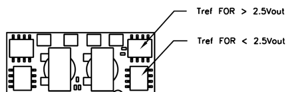
Figure 35. T ref Temperature measurement location.
