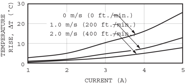
Figure 1. Typical Case Temperature Rise vs. Average Current (Case Temperature Must Be Kept Below 100 ^{\circ}\text{C} )
