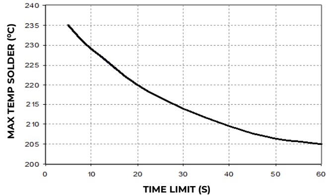
Figure 20. Time Limit, T_{lim} , Curve Above 205°C Reflow.
