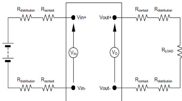
Figure 9. Output Voltage and Efficiency Test Setup.
