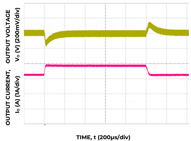
Figure 4. Transient Response to 0.1A/μs Dynamic load Change from 50% to 75% to 50% of full load, V_{in}=24V , C_o>100\mu F
