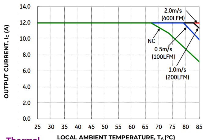
Figure 14. Output Current Derating for the Open Frame KHHD015A0F in the Transverse Orientation; Airflow Direction from Vin(+) to Vin(-); Vin = 24V.
