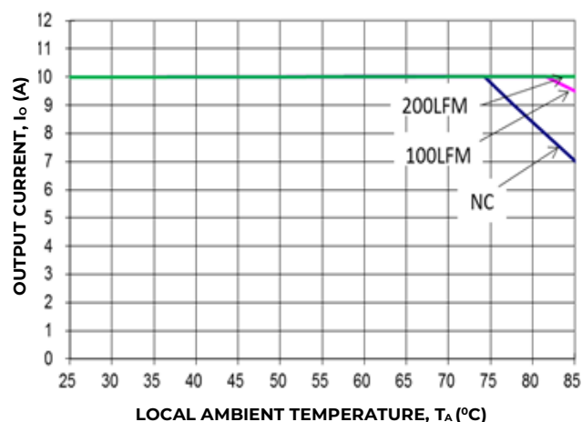
Figure 14. Output Current Derating for the Open Frame KHHD010A0F in the Transverse Orientation; Airflow Direction from Vin(+) to Vin(-); Vin = 24V.
