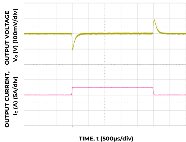
Figure 4. Transient Response to 0.1A/μS Dynamic Load Change from 50% to 75% to 50% of full load, V_{in}=48V
