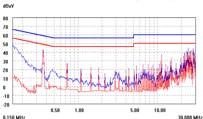
Figure 18. EMC signature using above filter, KHHD006A0A.
