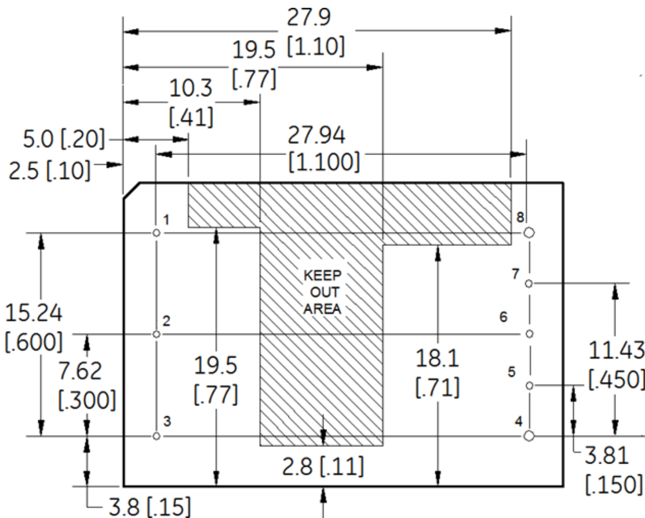
Pad Layout
