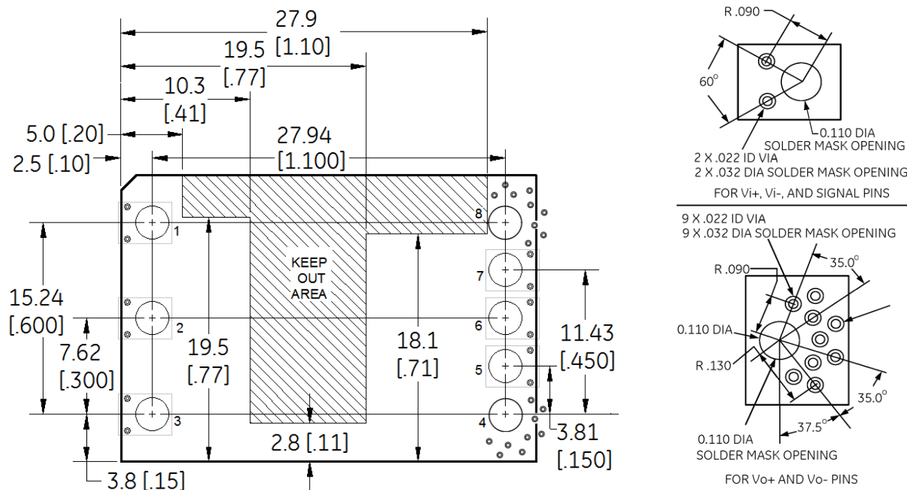
Surface Mount Pad Layout
