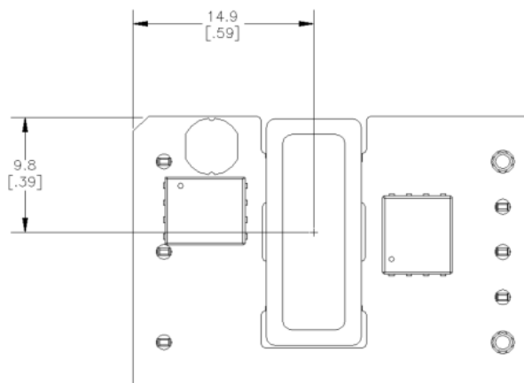
Figure 17. Pick and Place Location.
