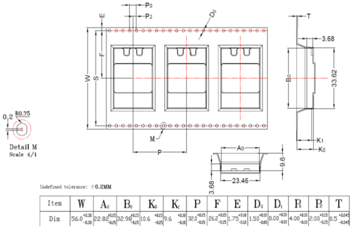
Surface Mount Module Tape & Reel Package
