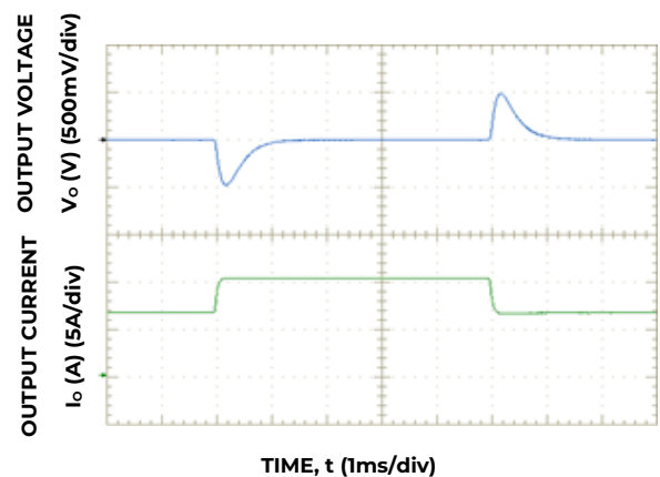
Figure 6. Dynamic Load Change Transient Response from 50% to 75% to 50% of Full Load at Room Temperature and 48V_{IN} ; 0.1A/\mu s , C_{o,ext} = 440\mu F .
