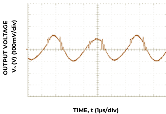
Figure 2. Typical output ripple and Noise at Room Temperature and 48V_{IN} ; I_o = I_{o,max} ; C_{o,ext} = 440\mu F .
