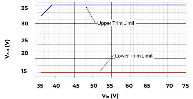
Figure 12. Output Voltage Trim Limits vs. Input Voltage.
