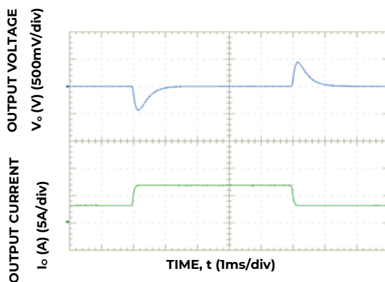
Figure 3. Dynamic Load Change Transient Response from 25% to 50% to 25% of Full Load at Room Temperature and 48V_{IN} ; 0.1A/\mu s , C_{o,ext} = 440\mu F .
