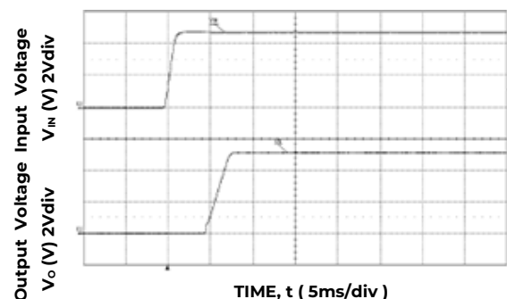
Figure 2. Typical Start-up using Input Voltage (V IN =12V, V out = V out , max, I out = I out , max)
