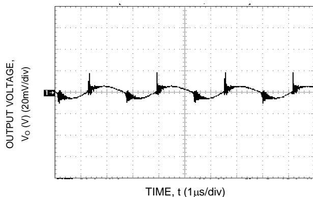
Figure 56. Typical Output Ripple and Noise.
